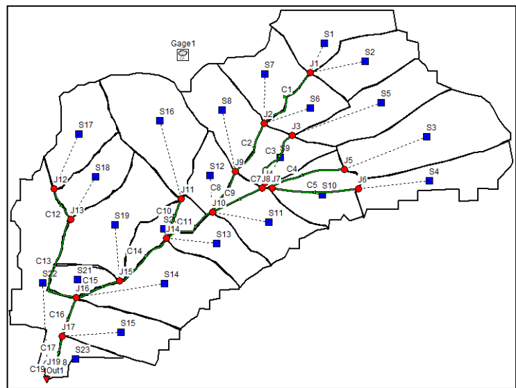
Figure 2 Sub basins, Channels, Junctions and gage station.
