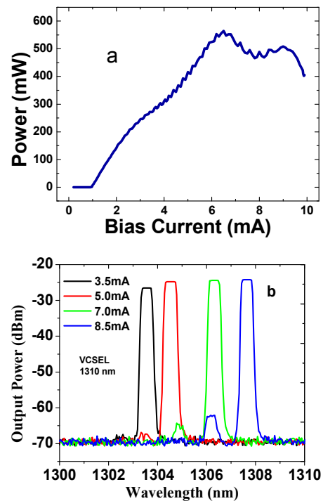
Figure 2. (a) Un-modulated VCSEL bias characteristics (b) VCSEL tune ability.
